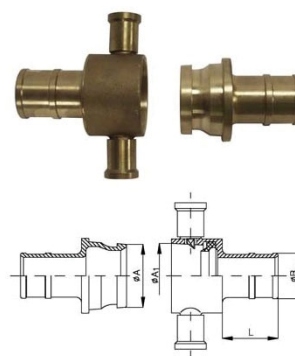
BS336 Coupling in Brass & Aluminum
