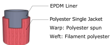
Single Jacket Hose
